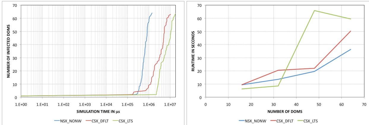
Figure 4 Infection propagation curve for 64-DOM (left) and runtime curves for 16, 32, 48 and 64 DOM scenarios (right) for cyber security benchmarks involving both CSX setups and, NSX without network control setup
