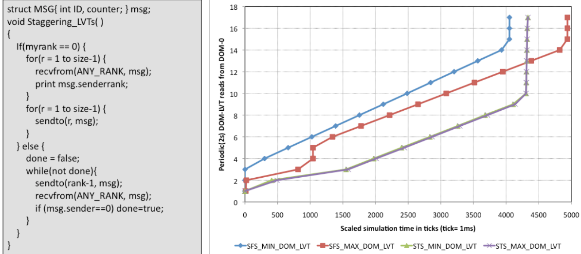
Figure 1 Algorithm to test staggering virtual timelines (left); Experiment results comparing simulation time divergence in SFS and STS (right).
