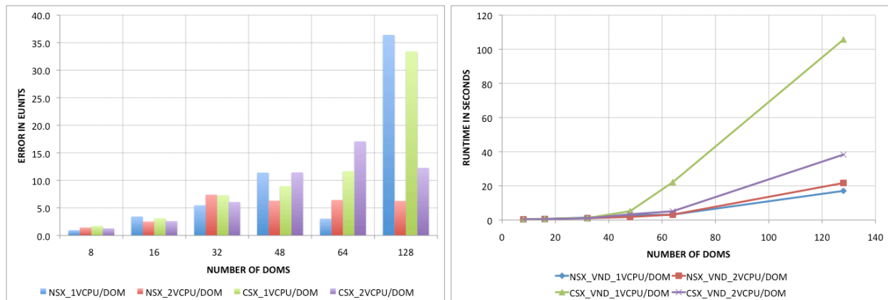
Figure 3 VND benchmark error plots (left); VND benchmark runtime plots (right)
