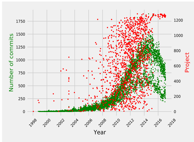
Figure 67: Time series of commit counts for the entire time frame (1998-2017) with project start date overlay
