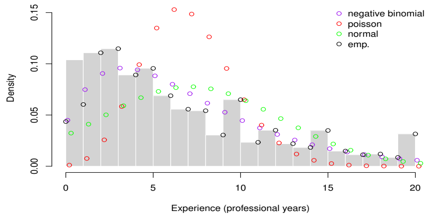
Figure 30: Histogram and distribution densities for professional coding years 0-20
