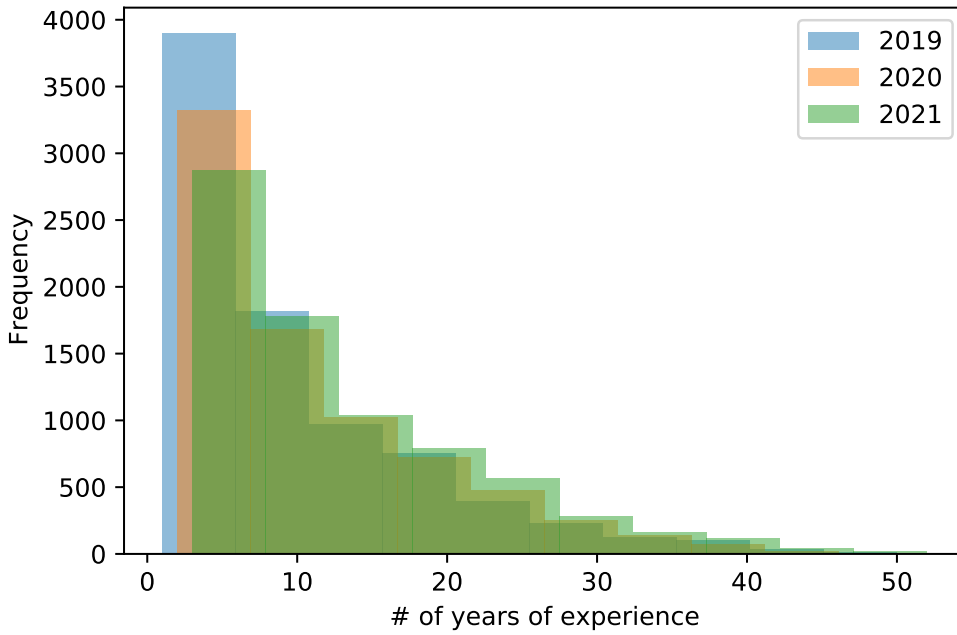
Figure 50: Histogram of all non-professional coders in 2019, 2020 and 2021
