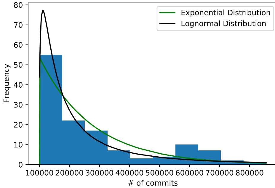
Figure 7: Histogram number of commits greater than 100K
