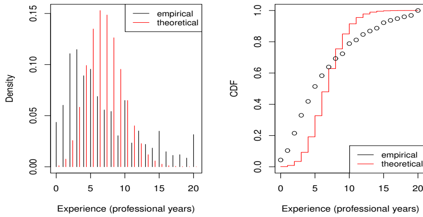
Figure 26: Density (left) and CDF (right) of empirical (data set) and Poisson distribution for professional coding years 0-20
