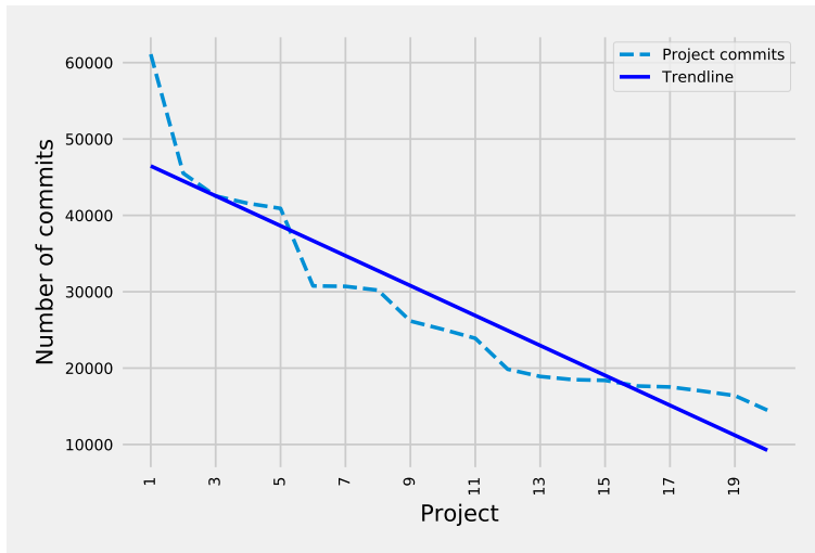
Figure 52: Project commits with trend line for top 20 projects
