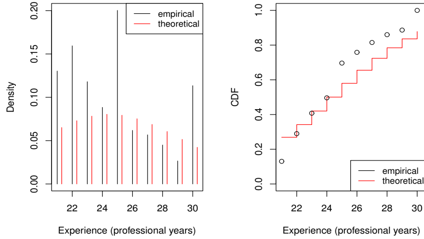
Figure 35: Density (left) and CDF (right) of empirical (data set) and Negative Binomial distribution for professional coding years 21-30
