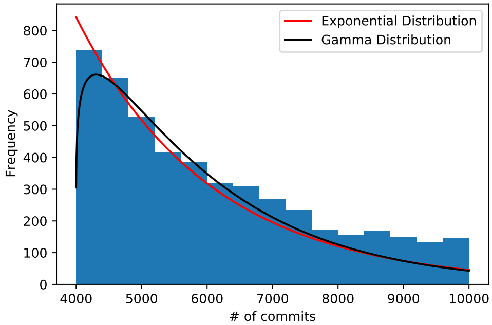
Figure 5: Histogram number of commits between 4K and 10K
