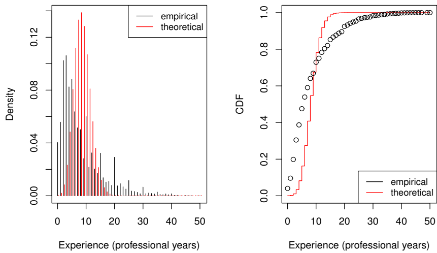
Figure 18: Density (left) and CDF (right) of empirical (data set) and Poisson distribution for professional coding years 0-50
