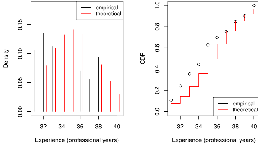
Figure 41: Density (left) and CDF (right) of empirical (data set) and Normal distribution for professional coding years 31-40
