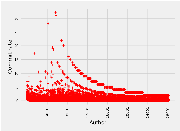
Figure 63: Author-level commit rates
