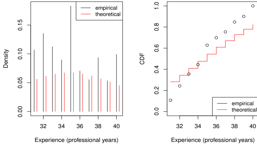
Figure 42: Density (left) and CDF (right) of empirical (data set) and Poisson distribution for professional coding years 31-40
