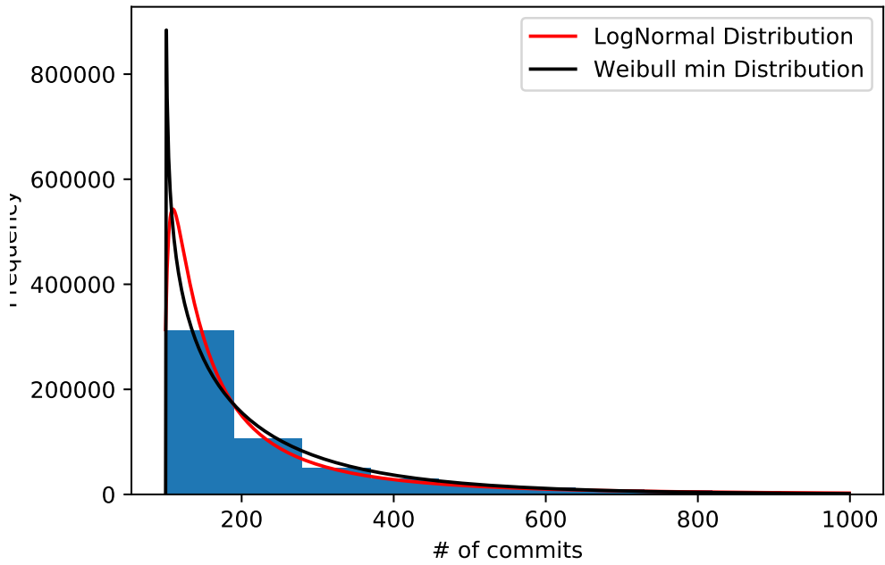
Figure 3: Histogram of number of commits between 100 and 1K
