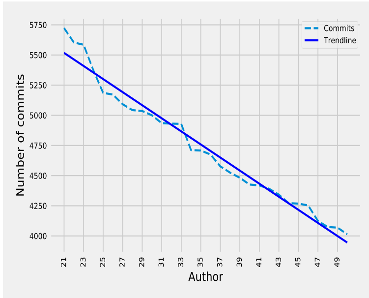
Figure 60: Commit authors with trend line for top 21-50 authors
