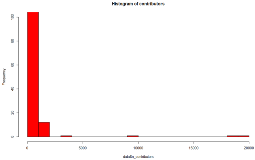
Figure 10: Histogram of the numbers of contributors to the repositories
