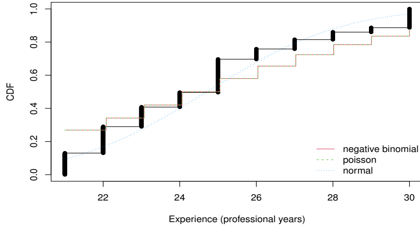
Figure 37: CDF plot of Normal, Poisson and Negative Binomial distribution along with empirical distribution (data set) for professional coding years 21-30
