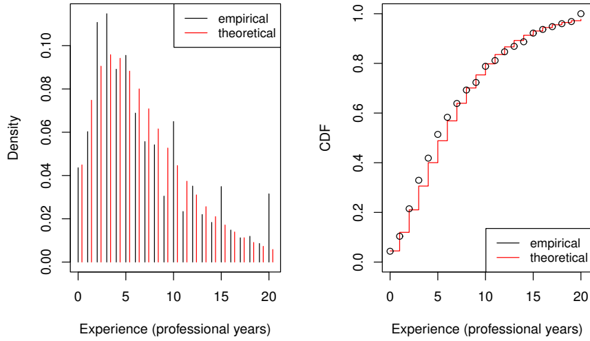
Figure 27: Density (left) and CDF (right) of empirical (data set) and Negative Binomial distribution for professional coding years 0-20
