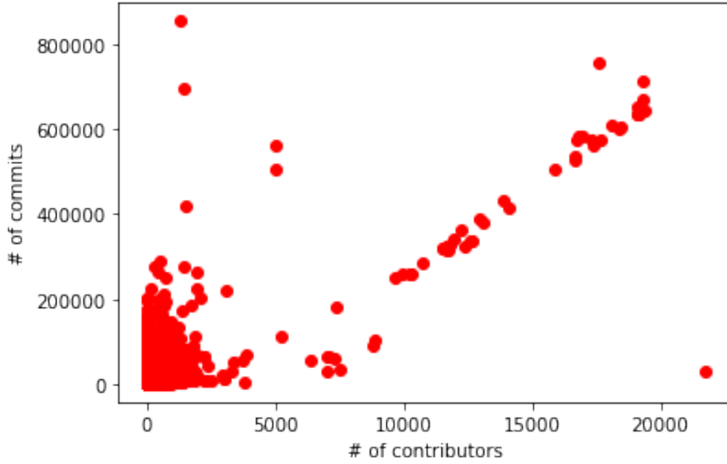
Figure 9: Number of Commits vs Number of Contributors
