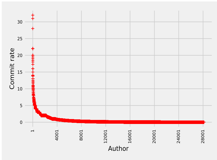
Figure 64: Author-level commit rates (high-low)
