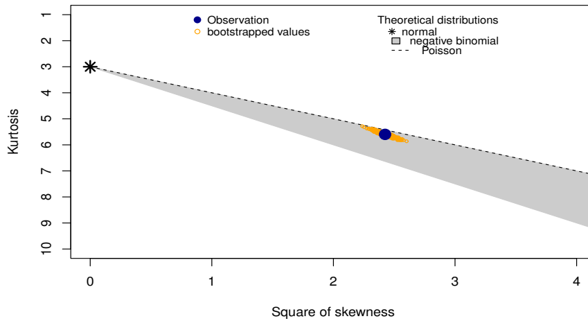
Figure 16: Skewness-kurtosis plot of professional coding years (0-50)
