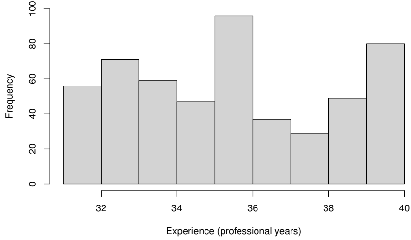
Figure 39: Frequency histogram of professional coding years (31-40)
