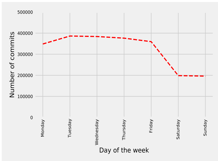
Figure 65: Weekly commit trend for total number of commits
