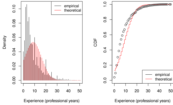
Figure 17: Density (left) and CDF (right) of empirical (data set) and Normal distribution for professional coding years 0-50
