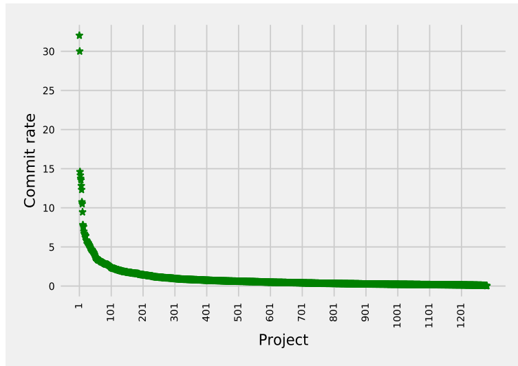
Figure 57: Project-level commit rate (high-low)
