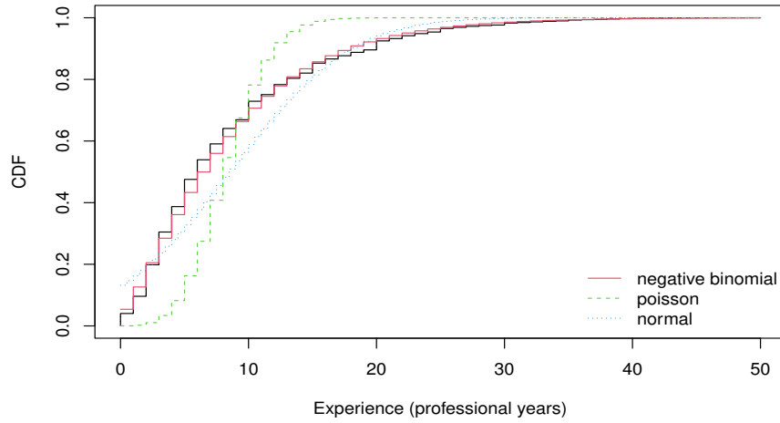
Figure 21: CDF plot of Normal, Poisson and Negative Binomial distribution along with empirical distribution (data set) for professional coding years 0-50
