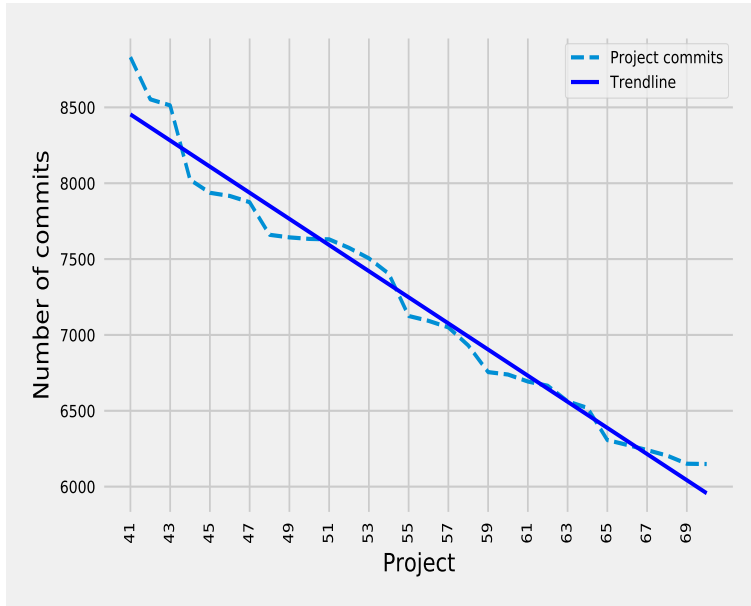
Figure 54: Project commits with trend line for top 41-70 projects
