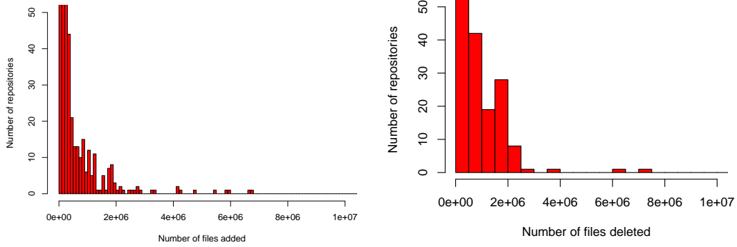
Figure 68: Histograms of additions (left) and deletions (right) of files
