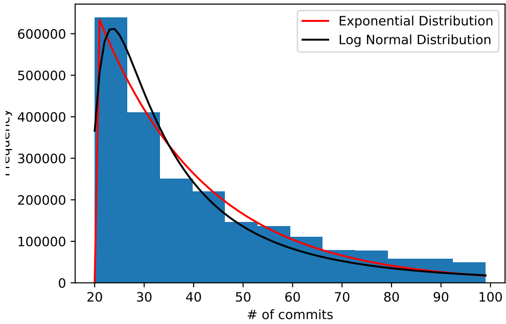
Figure 2: Histogram of number of commits between 20 and 100
