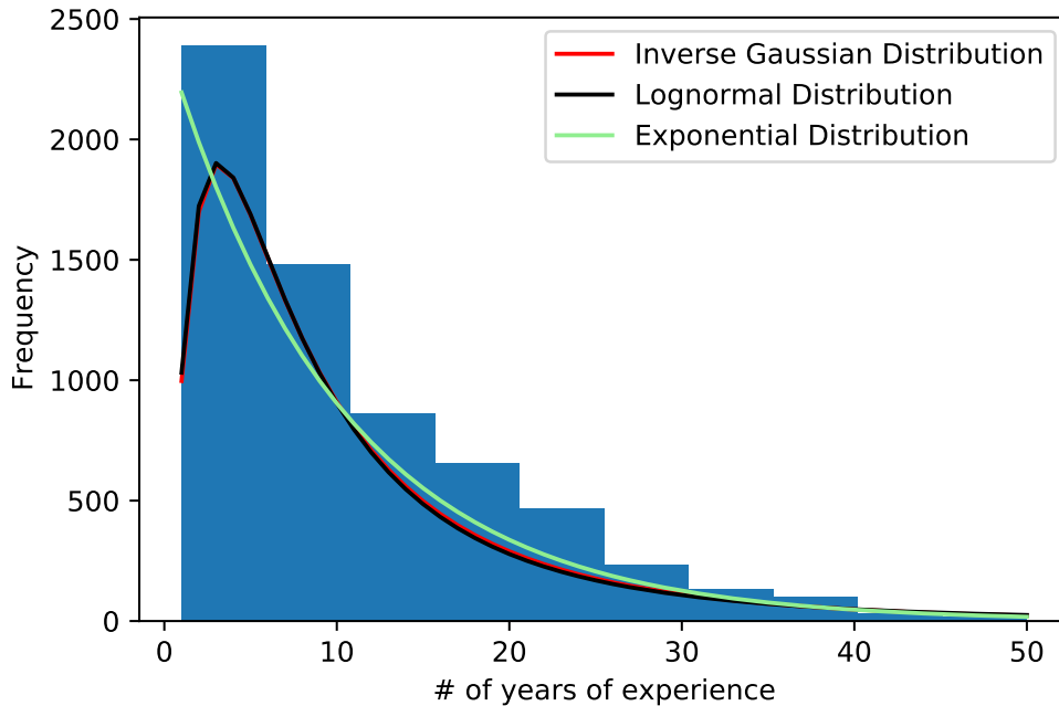
Figure 14: Histogram of non-professional coders
