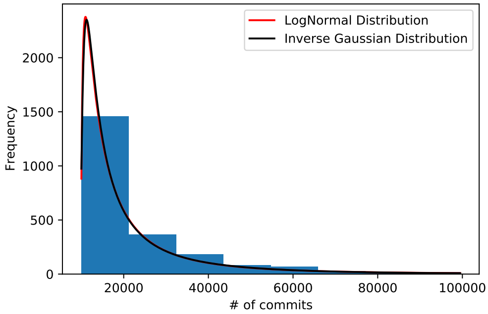
Figure 6: Histogram number of commits between 10K and 100K
