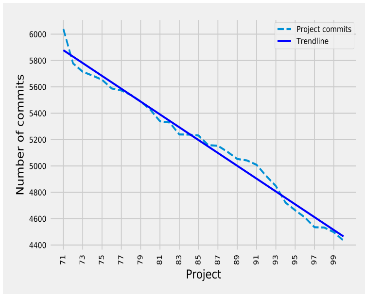
Figure 55: Project commits with trend line for top 71-100 projects
