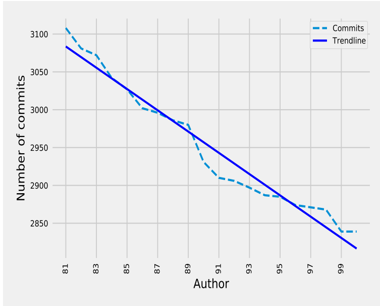
Figure 62: Commit authors with trend line for top 81-100 authors
