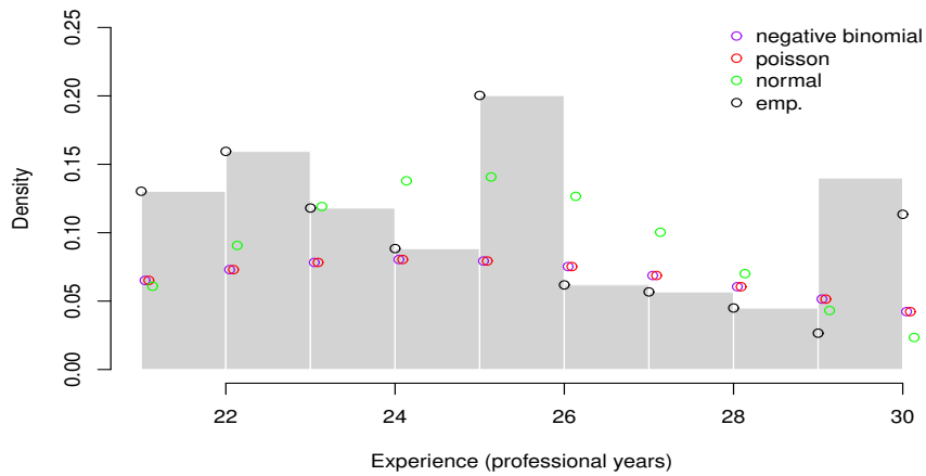
Figure 38: Histogram and distribution densities for professional coding years 21-30
