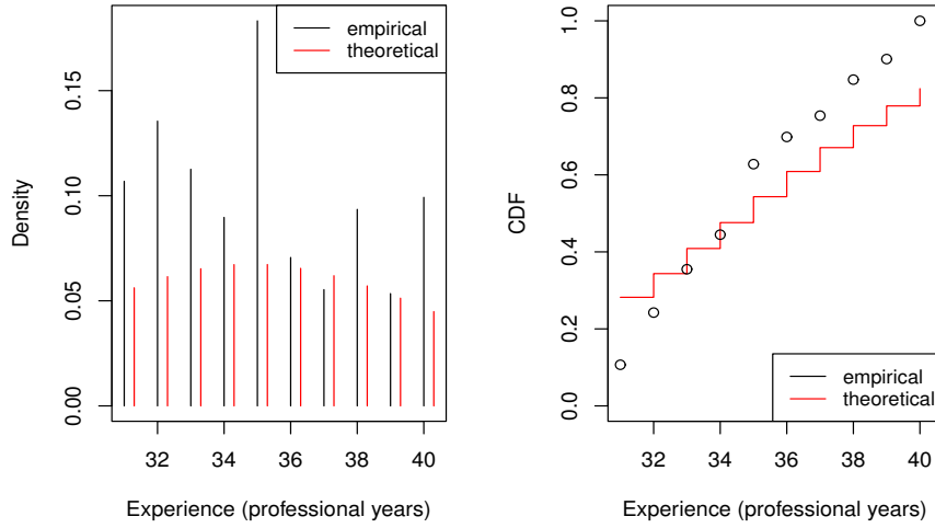
Figure 43: Density (left) and CDF (right) of empirical (data set) and Negative Binomial distribution for professional coding years 31-40
