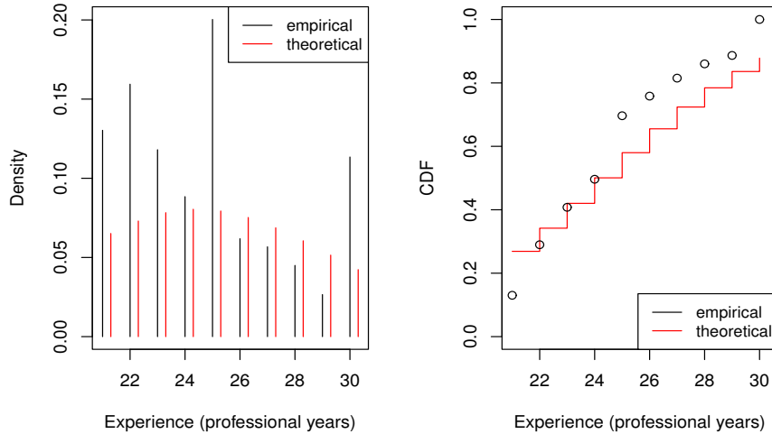
Figure 34: Density (left) and CDF (right) of empirical (data set) and Poisson distribution for professional coding years 21-30
