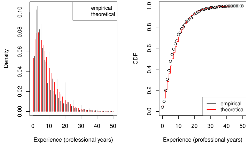
Figure 19: Density (left) and CDF (right) of empirical (data set) and Negative Binomial distribution for professional coding years 0-50
