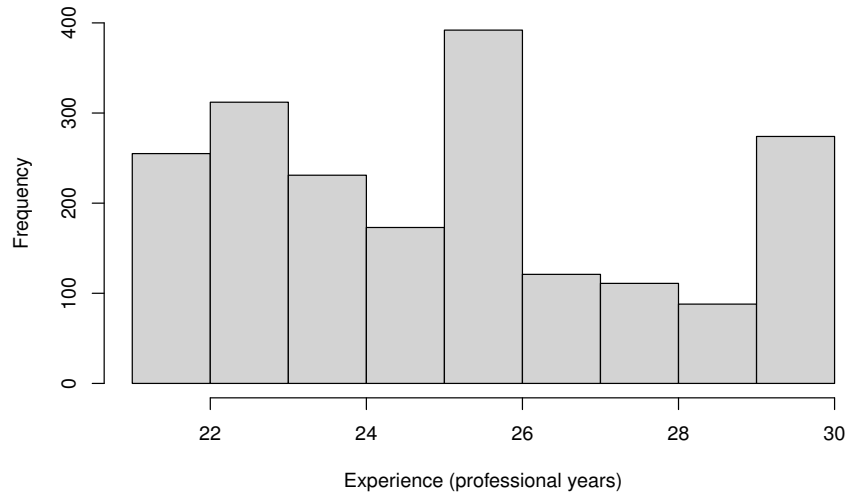
Figure 31: Frequency histogram of professional coding years (21-30)
