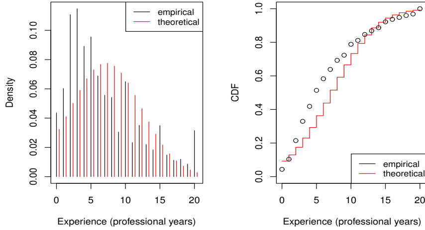
Figure 25: Density (left) and CDF (right) of empirical (data set) and Normal distribution for professional coding years 0-20
