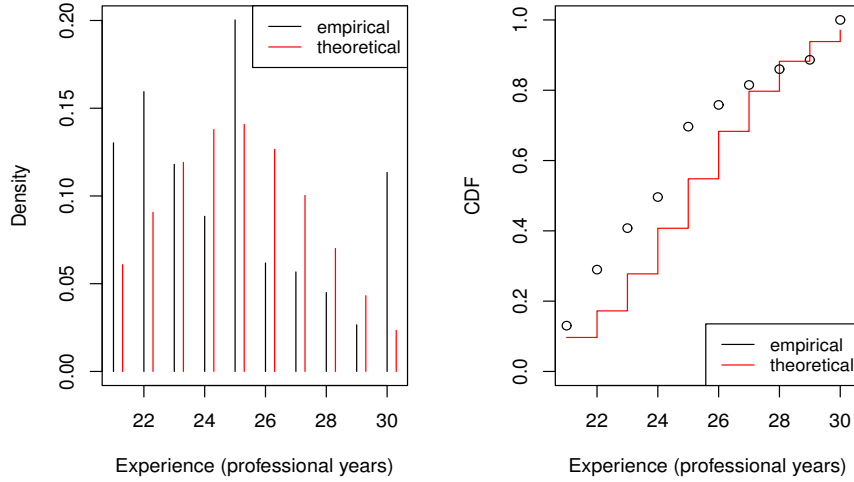
Figure 33: Density (left) and CDF (right) of empirical (data set) and Normal distribution for professional coding years 21-30
