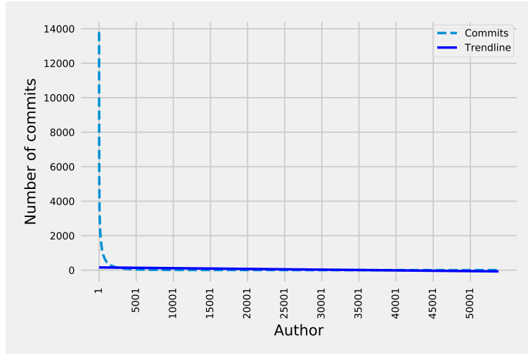
Figure 58: Commit authors with trend line
