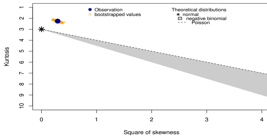
Figure 32: Skewness-kurtosis plot of professional coding years (21-30)
