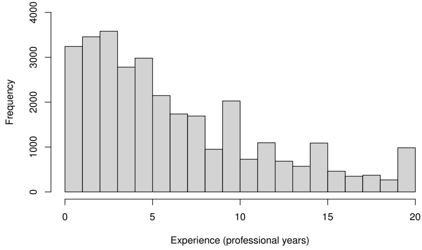
Figure 23: Frequency histogram of professional coding years (0-20)
