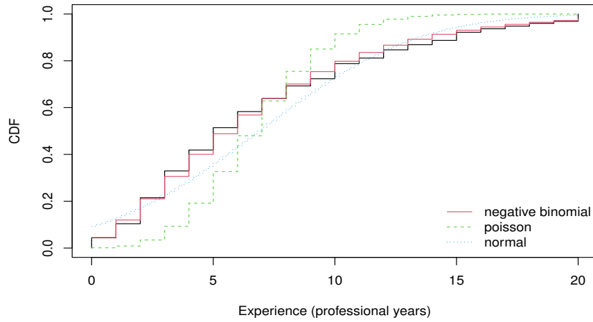
Figure 29: CDF plot of Normal, Poisson and Negative Binomial distribution along with empirical distribution (data set) for professional coding years 0-20
