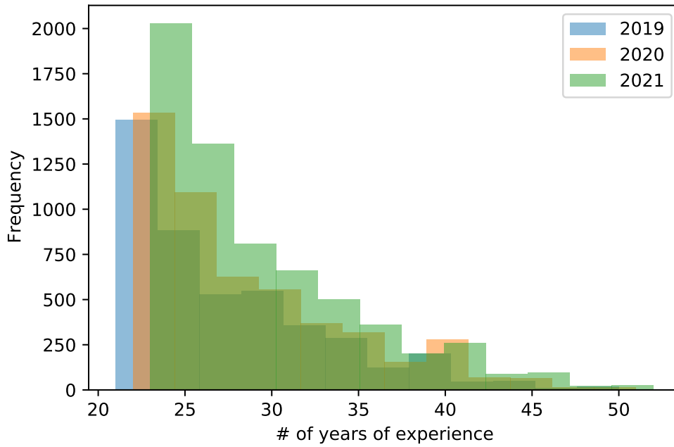
Figure 48: Histogram of professional coders in 2019, 2020 and 2021 between 20 and 50 years of experience
