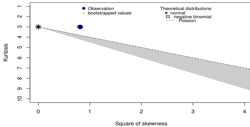
Figure 24: Skewness-kurtosis plot of professional coding years (0-20)
