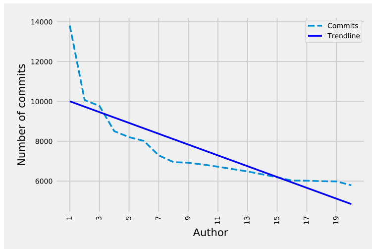
Figure 59: Commit authors with trend line for top 20 authors
