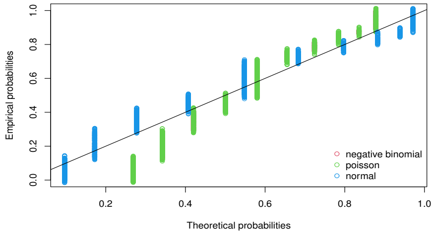
Figure 36: P-P plot of Normal, Poisson and Negative Binomial distribution along with empirical distribution (data set) for professional coding years 21-30
