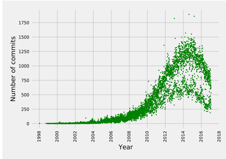
Figure 66: Time series of commit counts for the entire time frame (1998-2017)
