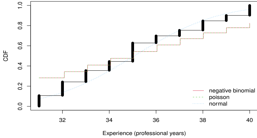
Figure 45: CDF plot of Normal, Poisson and Negative Binomial distribution along with empirical distribution (data set) for professional coding years 31-40
