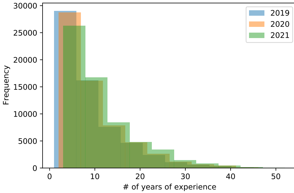
Figure 49: Histogram of all professional coders in 2019, 2020 and 2021
