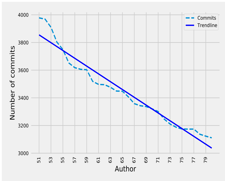
Figure 61: Commit authors with trend line for top 51-80 authors
