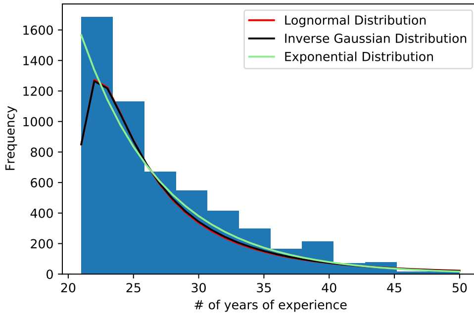
Figure 12: Histogram of professional coders with more than 20 years of experience
