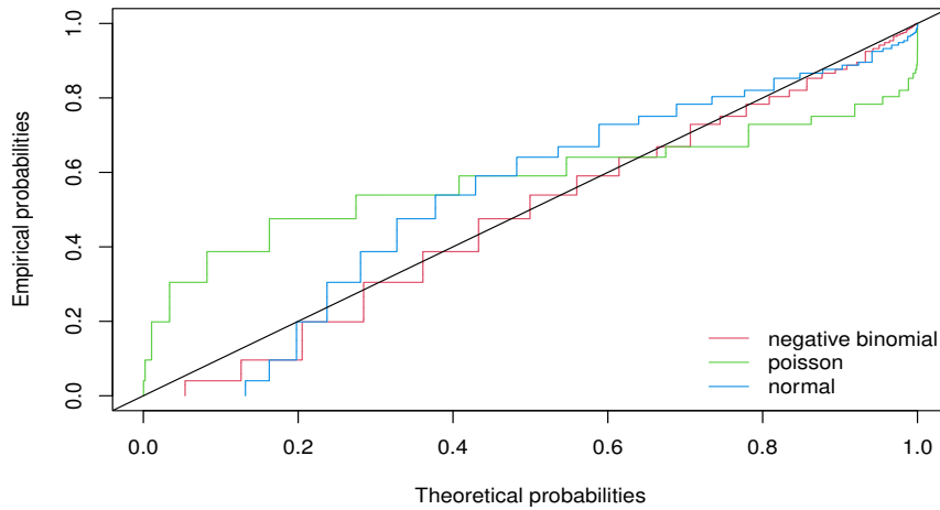
Figure 20: P-P plot of Normal, Poisson and Negative Binomial distribution along with empirical distribution (data set) for professional coding years 0-50
