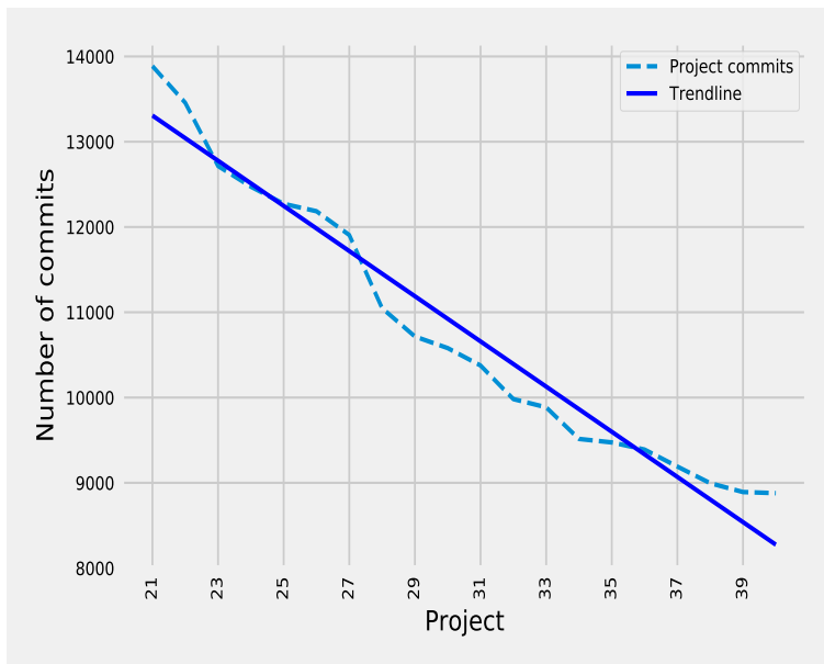
Figure 53: Project commits with trend line for top 21-40 projects
