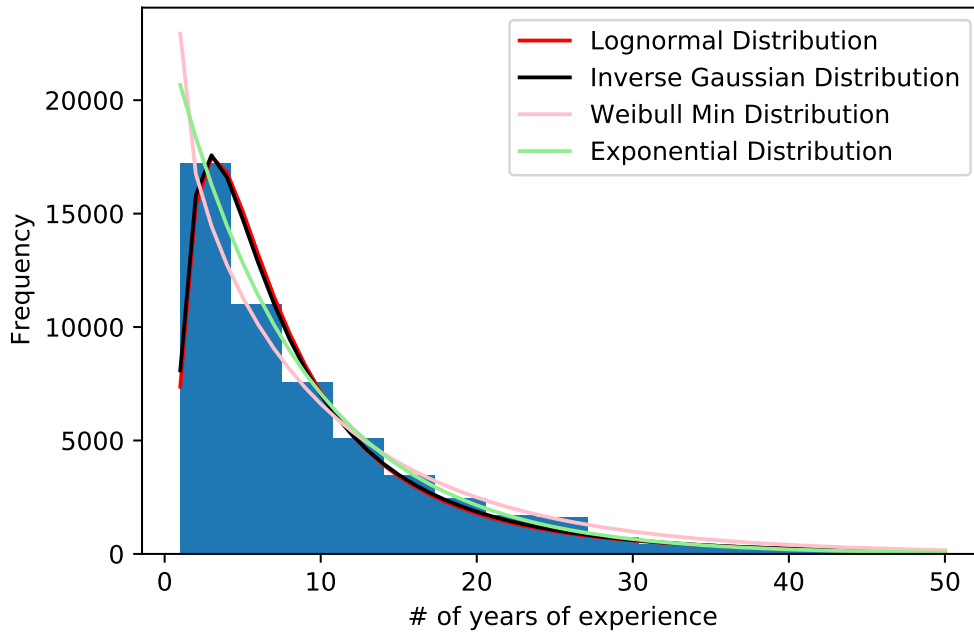
Figure 13: Histogram of all the professional coders
