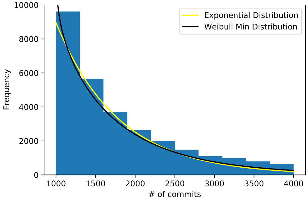
Figure 4: Histogram of number commits between 1K and 4K
