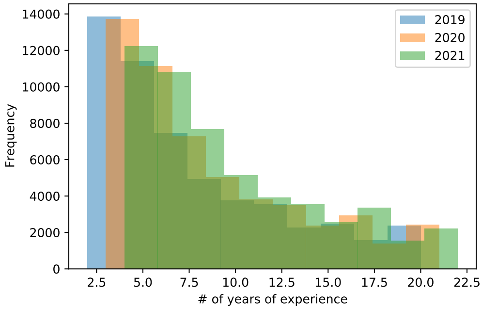
Figure 47: Histogram of professional coders in 2019, 2020 and 2021 with upto 20 years of experience
