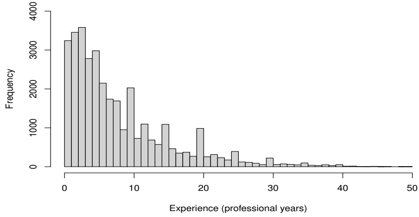
Figure 15: Frequency histogram of professional coding years (0-50)
