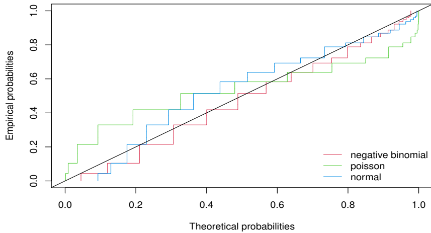
Figure 28: P-P plot of Normal, Poisson and Negative Binomial distribution along with empirical distribution (data set) for professional coding years 0-20
