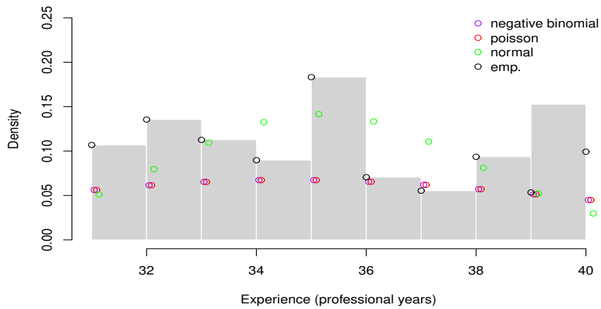
Figure 46: Histogram and distribution densities for professional coding years 31-40
