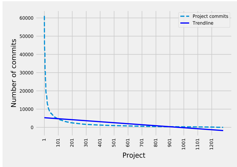
Figure 51: Project commits with trend line
