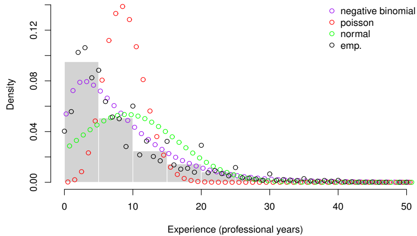
Figure 22: Histogram and distribution densities for professional coding years 0-50
