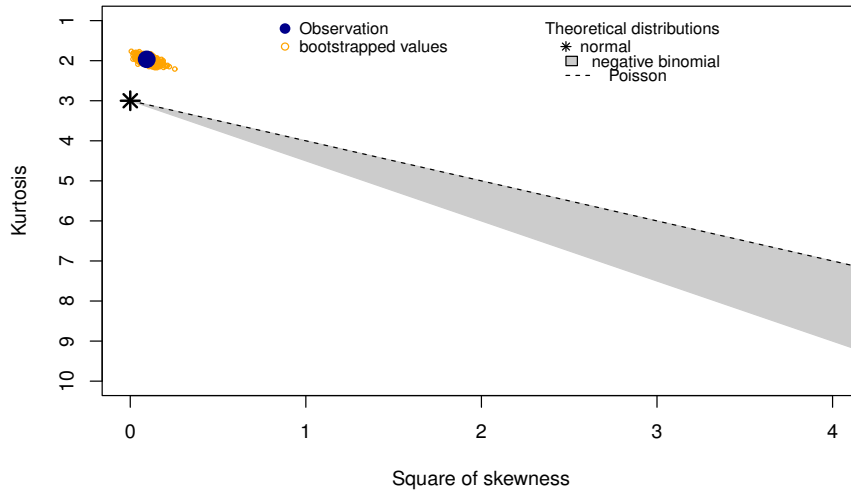
Figure 40: Skewness-kurtosis plot of professional coding years (31-40)
