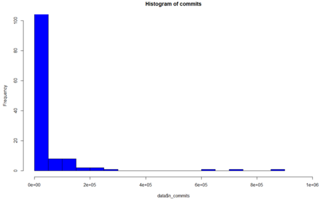
Figure 8: Histogram of all the commits to all repositories
