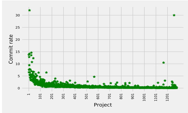
Figure 56: Project-level commit rate for 1281 projects
