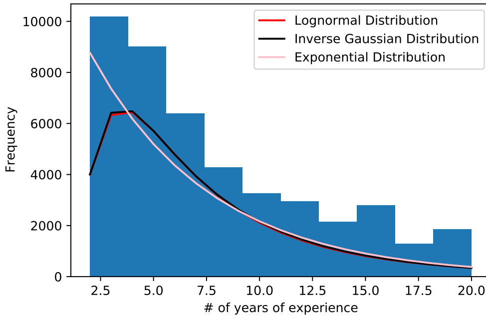
Figure 11: Histogram of professional coders between 2 and 20 years of experience
