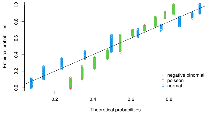
Figure 44: P-P plot of Normal, Poisson and Negative Binomial distribution along with empirical distribution (data set) for professional coding years 31-40
